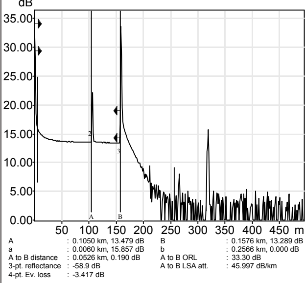
BEZEQINT HA-SIVIM_akvarium_A2-2_Fiber01_8...
