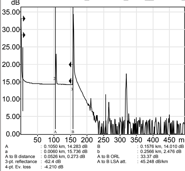
BEZEQINT HA-SIVIM_akvarium_A2-2_Fiber02_8...
