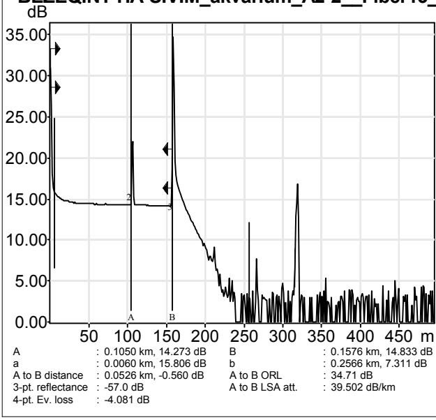
BEZEQINT HA-SIVIM_akvarium_A2-2_Fiber13_8...
