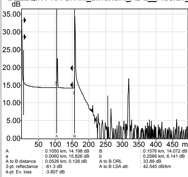
BEZEQINT HA-SIVIM_akvarium_A2-2_Fiber21_8...
