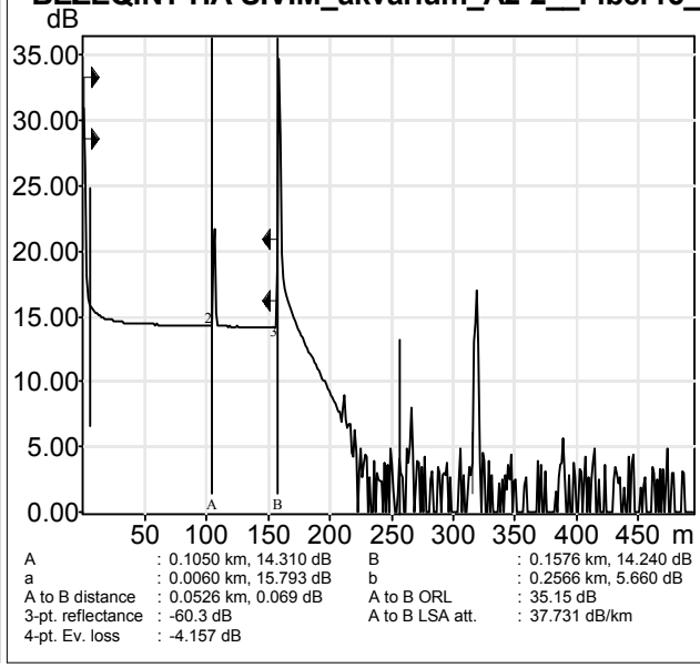
BEZEQINT HA-SIVIM_akvarium_A2-2_Fiber15_8...
