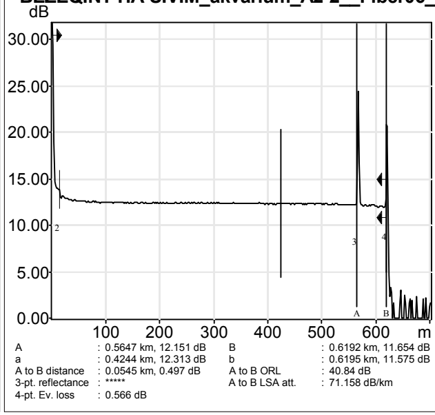
BEZEQINT HA-SIVIM_akvarium_A2-2_Fiber06_1...
