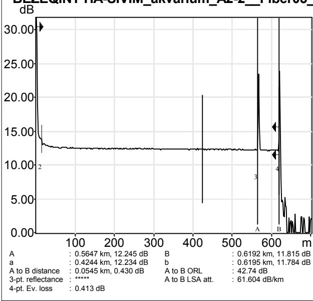
BEZEQINT HA-SIVIM_akvarium_A2-2_Fiber05_1...
