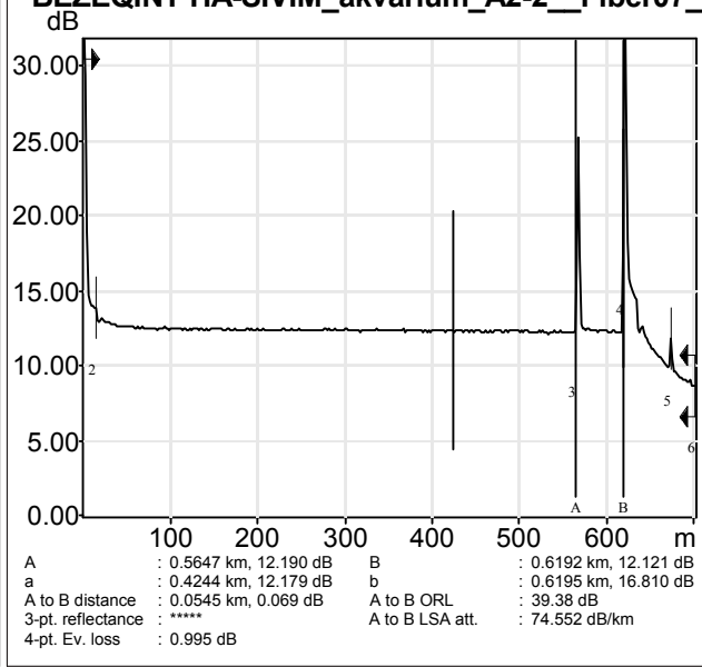
BEZEQINT HA-SIVIM_akvarium_A2-2_Fiber07_1...
