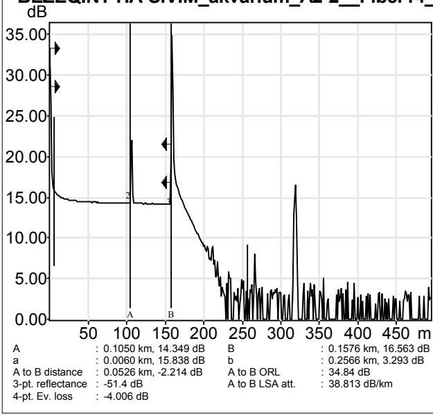
BEZEQINT HA-SIVIM_akvarium_A2-2_Fiber14_8...
