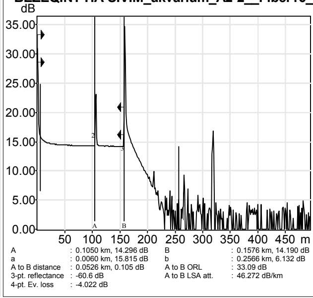
BEZEQINT HA-SIVIM_akvarium_A2-2_Fiber16_8...
