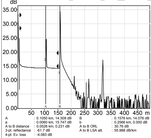
BEZEQINT HA-SIVIM_akvarium_A2-2_Fiber04_8...
