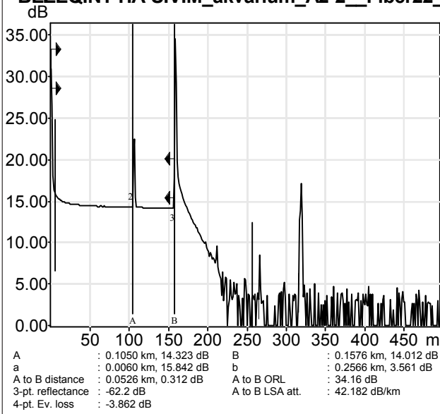
BEZEQINT HA-SIVIM_akvarium_A2-2_Fiber22_8...
